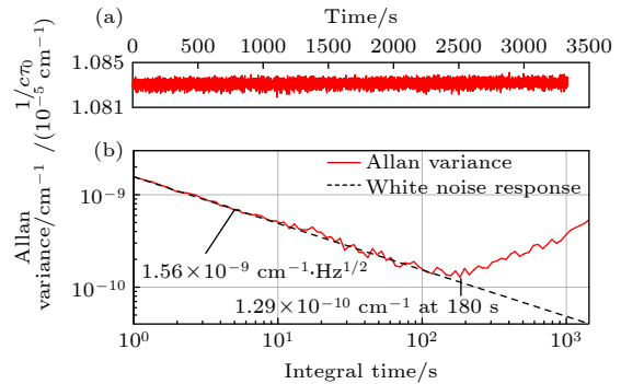
图 9 空腔衰荡时间的长期测量 (a) 和 Allan 方差分析 (b), 黑色点线为白噪声响应曲线, 红色曲线为 Allan 方差 Fig. 9. Long-term measurement of cavity ring-down time (a) and Allan variance analysis (b). The black dotted line is the white noise response curve, and the red curve is the Allan variance.
