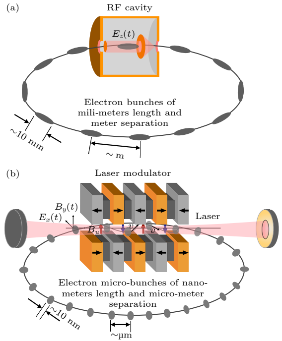
图 2 SSMB 储存环 (b) 与传统储存环 (a) 对比 Fig. 2. Comparison between an SSMB storage ring (b) with a conventional storage ring (a).
