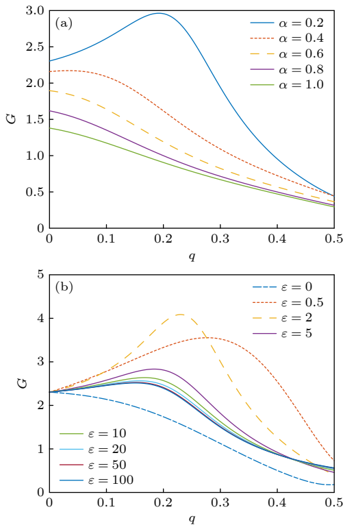
图 2 系统输出幅值增益随噪声稳态转移概率 q 变化的 GSR 现象, 其中 m = 1, \gamma = 0.1, \omega = 1, \Omega = 1.4, \lambda = 0.1, a = 0.7 (a) \varepsilon = 4 ; (b) \alpha = 0.2 Fig. 2. The OAG versus q with m = 1, \gamma = 0.1, \omega = 1, \Omega = 1.4, \lambda = 0.1, a = 0.7 : (a) \varepsilon = 4 ; (b) \alpha = 0.2 .
