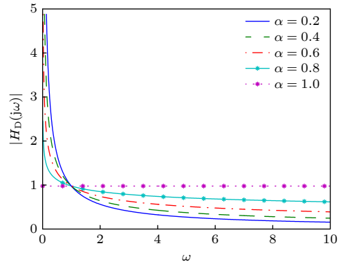
图 3 分数阶阻尼项的频率特征 Fig. 3. Frequency characteristics of the fractional damping term.
