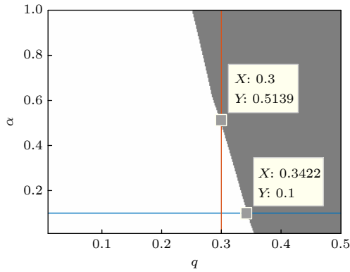
图 4 随 \varepsilon 变化的 GSR 现象在 q - \alpha 平面的相图, 其中 m = 1, \gamma = 0.1, \omega = 1, \Omega = 1.6, \lambda = 0.1, a = 0.4 Fig. 4. Phase diagram for GSR versus \varepsilon in the q - \alpha plane, with m = 1, \gamma = 0.1, \omega = 1, \Omega = 1.6, \lambda = 0.1, a = 0.4 .
