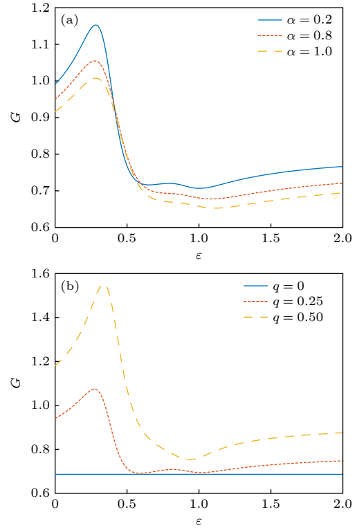
图 5 系统输出幅值增益随耦合系数 \varepsilon 变化的 GSR 现象, 其中 m = 1, \gamma = 0.1, \omega = 1, \Omega = 1.6, \lambda = 0.1, a = 0.4 (a) q = 0.3 ; (b) \alpha = 0.1 Fig. 5. The OAG versus \varepsilon with m = 1, \gamma = 0.1, \omega = 1, \Omega = 1.6, \lambda = 0.1, a = 0.4 : (a) q = 0.3 ; (b) \alpha = 0.1 .
