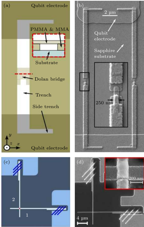
图 6 两种约瑟夫森结设计方案 (a), (c) 设计图; (b), (d) 对应设计图制备的约瑟夫森结电镜照片 [112,113] Fig. 6. Two designs of Josephson junctions: (a), (c) Design drawings; (b), (d) electron micrographs of Josephson junctions prepared by corresponding designs [112,113].
