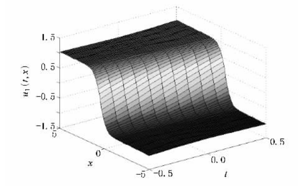
图6 u_1(t, x) 的曲面图( p = q = 1, \beta = 0.9, x_0 = 0 )
