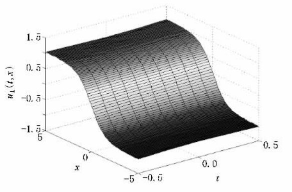
图4 u_1(t, x) 的曲面图( p = q = 1, \beta = 0.1, x_0 = 0 )
