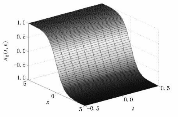
图3 u_0(t, x) 的曲面图( p = q = 1, \beta = 0.1, x_0 = 0 )
