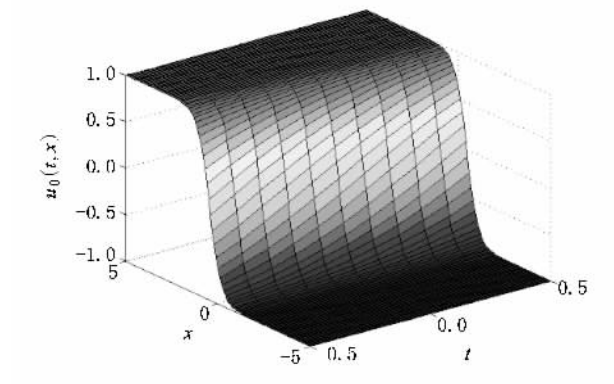
图5 u_0(t, x) 的曲面图( p = q = 1, \beta = 0.9, x_0 = 0 )
