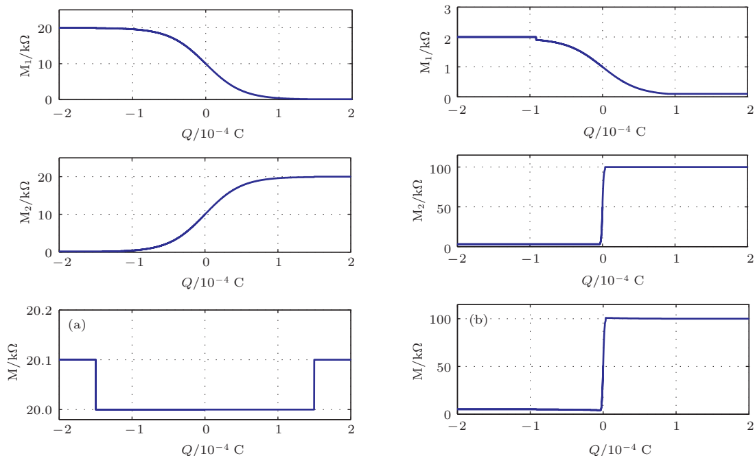
图 11 两个忆阻器反向串联时忆阻值和电荷量之间的关系 (a) Case 13, 其中 R_{on1} = 100 \Omega , R_{off1} = 20000 \Omega , R_{on2} = 100 \Omega , R_{off2} = 20000 \Omega ; (b) Case 1, 其中 R_{on1} = 80 \Omega , R_{off1} = 2000 \Omega , R_{on2} = 3000 \Omega , R_{off2} = 100000 \Omega
