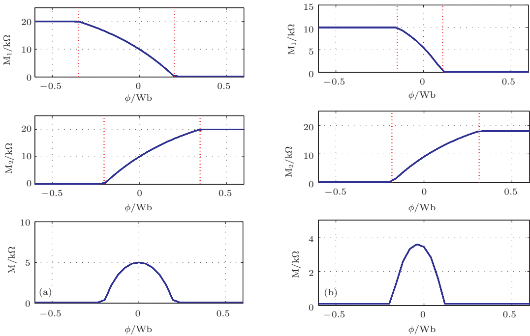
图 21 (网刊彩色) 两个忆阻器反向并联时忆阻值和磁通量之间的关系 (a) Case 1, 其中 R_{on1} = 100 \Omega , R_{off1} = 20000 \Omega , R_{on2} = 100 \Omega , R_{off2} = 20000 \Omega , \mu_{v1} = \mu_{v2} = 10^{-14} \text{ m}^2 \cdot \text{s}^{-1} \cdot \text{V}^{-1} ; (b) Case 7, 其中 R_{on1} = 100 \Omega , R_{off1} = 10000 \Omega , R_{on2} = 100 \Omega , R_{off2} = 18000 \Omega , \mu_{v1} = \mu_{v2} = 10^{-14} \text{ m}^2 \cdot \text{s}^{-1} \cdot \text{V}^{-1}
