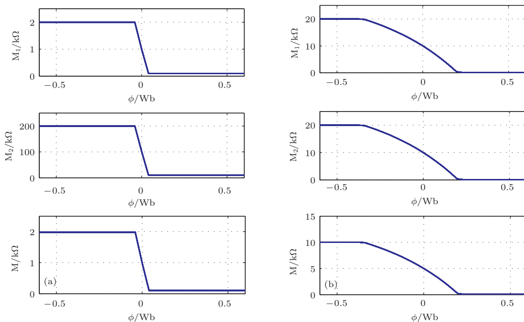
图 12 电压与忆阻器极性一致时两个忆阻器同向并联时忆阻值和磁通量之间的关系 (a) Case 1, 其中 R_{on1} = 100 \Omega , R_{off1} = 2000 \Omega , R_{on2} = 9800 \Omega , R_{off2} = 200000 \Omega ; (b) Case 13, 其中 R_{on1} = 100 \Omega , R_{off1} = 20000 \Omega , R_{on2} = 100 \Omega , R_{off2} = 20000 \Omega
