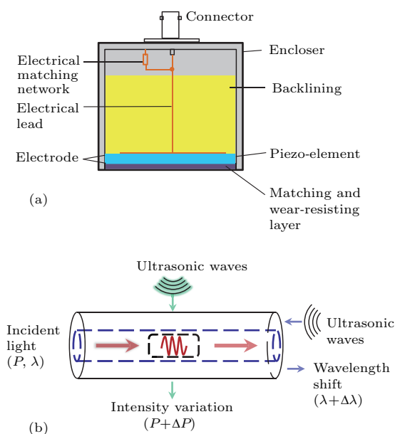
图 1 (a) PZT; (b) 光纤超声传感器传感机理 Fig. 1. Sensing mechanisms: (a) PZT; (b) fiber-optics ultrasonic sensor.
