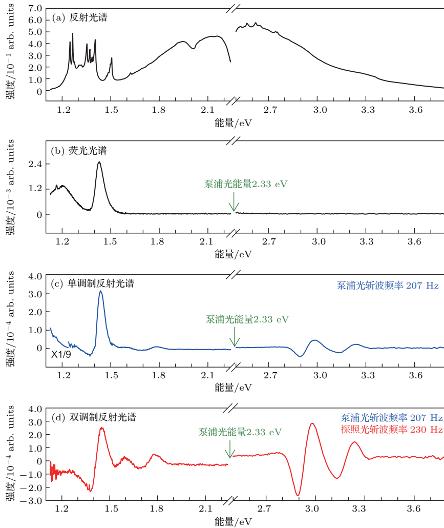
图2 半绝缘(001) GaAs体材料在探测范围为1.1—3.8 eV内的反射光谱(a), 泵浦激光光子能量为2.33 eV(532 nm)时的荧光光谱(b), 单调制反射光谱(c)以及双调制反射光谱(d); 泵浦激光斩波频率为207 Hz, 探测光斩波频率为230 Hz Fig. 2. (a) Reflectance, (b) photoluminescence, (c) single-modulated photoreflectance and (d) dual-modulated photoreflectance of semi-insulating GaAs (001) in the range of 1.1 eV to 3.8 eV. For the photoluminescence, the photon energy of the pumping laser is 2.33 eV. For photoreflectance, the pumping laser is chopped at f_1 = 207 Hz and the probing light is chopped at f_2 = 230 Hz.
