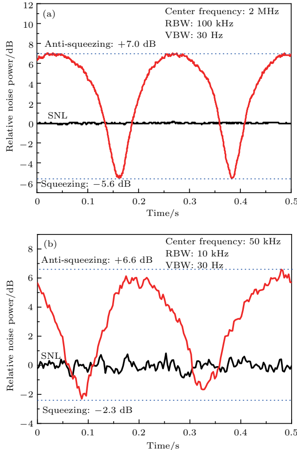
图3 扫描 LO 光与压缩真空的相对位相时得到的压缩谱 (a), (b) 分别为分析频率为 2 MHz 和 50 kHz 的结果 Fig. 3. Squeezing traces with the scanning of the relative phase between LO and the vacuum squeezing, the analysis frequencies are 2 MHz for (a) and 50 kHz for (b), respectively.
