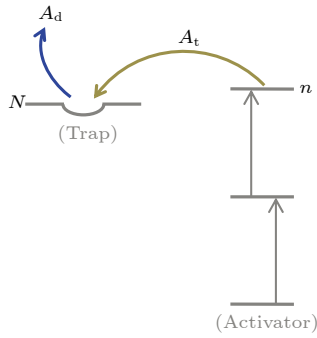
图1 考虑了光激励排空影响的上转换充能动力学示意图 Fig. 1. Schematic illustration of up-conversion charging dynamics. The population in traps depends on the competition between the trapping and excitation-light detrapping.
