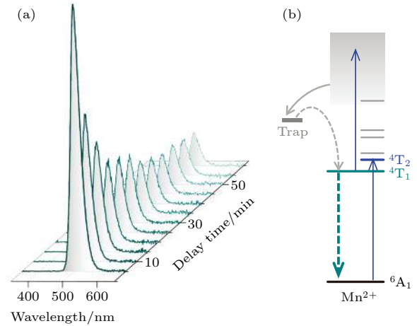
图2 LaMgGa 11 O 19 :Mn 2+ 材料的上转换充能余辉发射谱; (b) 上转换充能及伴随的余辉发射路径示意图 Fig. 2. (a) Up-conversion charging induced persistent luminescence (UCC-PersL) emission spectra of LaMgGa 11 O 19 :Mn 2+ ; (b) schematic representation of the UCC-PersL process.
