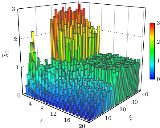
图 7 APD 恢复曲线总平均斜率 \bar{\lambda}_T 随参数 \beta, \gamma 变化的直方图 Fig. 7. Histogram of total average slope of APD restitution curve varying with parameters \beta and \gamma .
