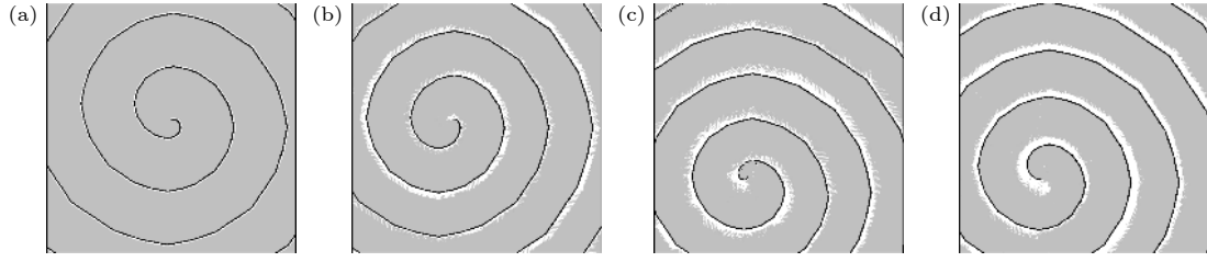
图 2 在参数 \alpha = 40 , \gamma = 10 , \beta = 14 下不同时刻的膜电位斑图 (a) t = 0 ; (b) t = 20000 ; (c) t = 60000 ; (d) t = 100000 Fig. 2. Patterns of the membrane potential at different time moments for \alpha = 40 , \gamma = 10 and \beta = 14 : (a) t = 0 ; (b) t = 20000 ; (c) t = 60000 ; (d) t = 100000 .
